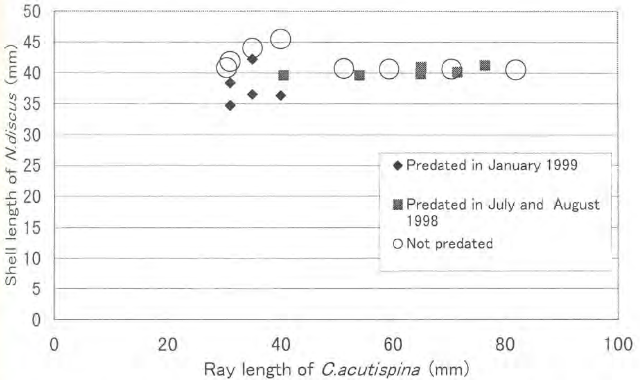
Fig. 3 Relation between ray length of predator, Coscinasterias acutispina , and shell length of preyed or surviving abalone (around the size of releasing), Nordotis discus hannai , in the feeding experiments.
